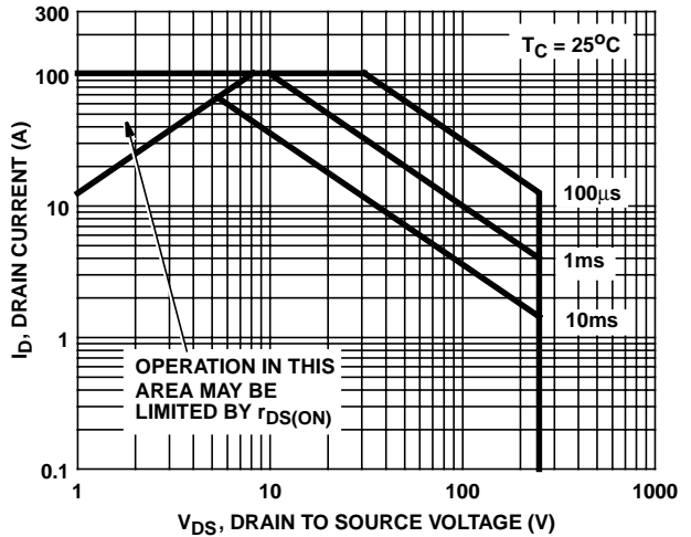
FIGURE 4. FORWARD BIAS SAFE OPERATING CURVE
