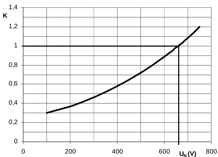
Fig. 1 i^2t coefficient multiplier vs. application voltage
