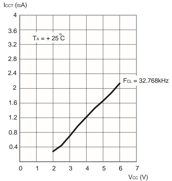
I CTT vs V CC
