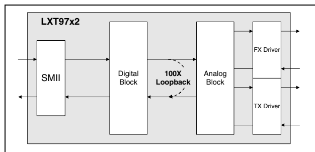
Figure 16. Loopback Paths
