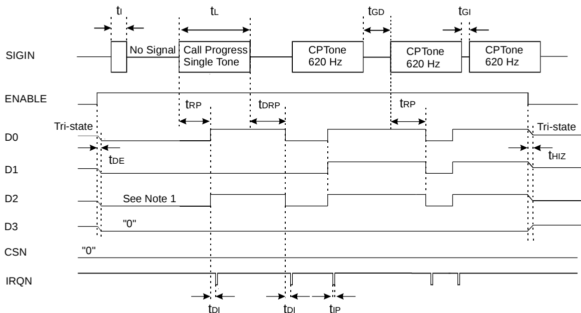
Figure 4 Timing Diagram: Call Progress Tone(s)
