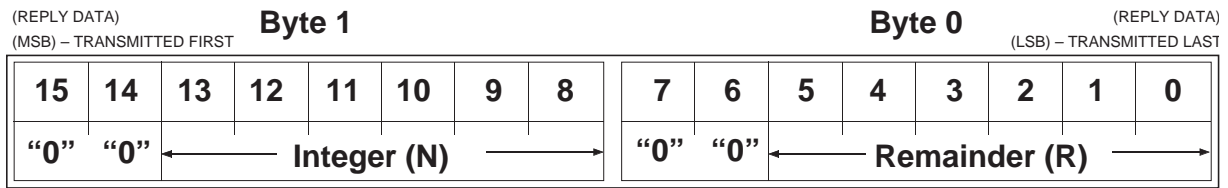
Fig. 6 Format of the CTCSS Rx Frequency Register
