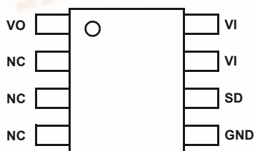
ISL9007 (8 Ld MSOP) TOP VIEW
