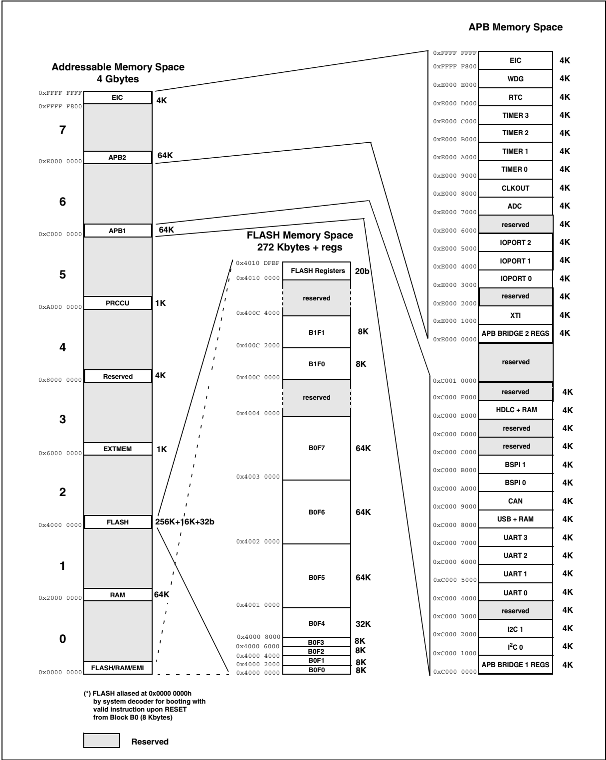
1.7 Memory Mapping Figure 6. Memory Map
