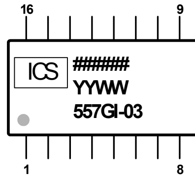
Marking Diagram (ICS557GI-03)
