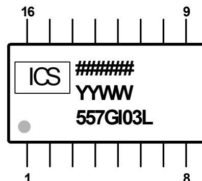
Marking Diagram (ICS557GI-03LF)
