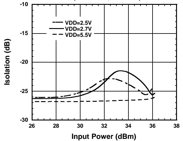
PC-P2 Isolation vs. Input Power ( PC-P1on, f=2GHz )
