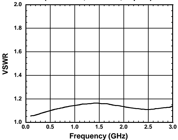
PC-P2 VSWR vs. Frequency ( VDD=2.7V, VCTL=0V, P2port )
