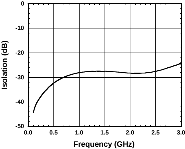
RX-ANT1 Isolation vs. Frequency
