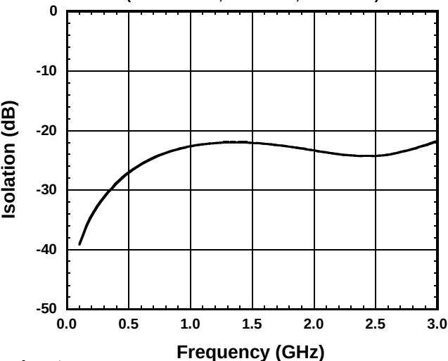
TX-ANT2 Isolation vs. frequency
