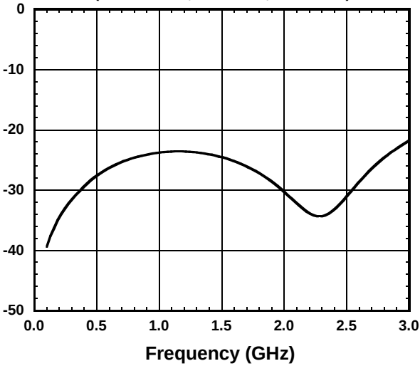
TX-ANT2 Isolation vs. frequency
