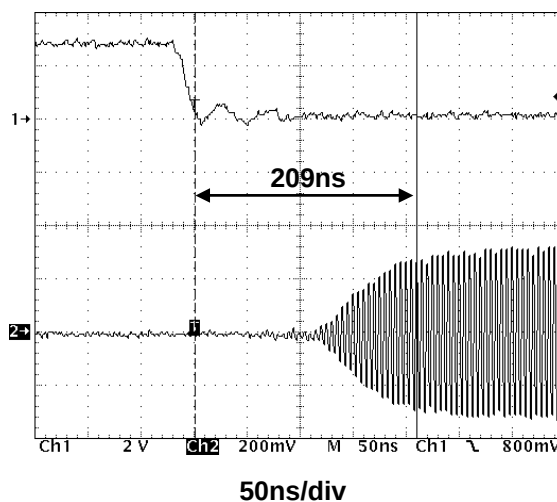
Switching Speed
