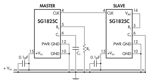
FIGURE 4. — OSCILLATOR SYNCHRONIZATION
