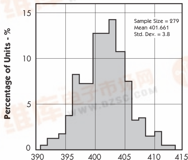
INITIAL OSCILLATOR ACCURACY
