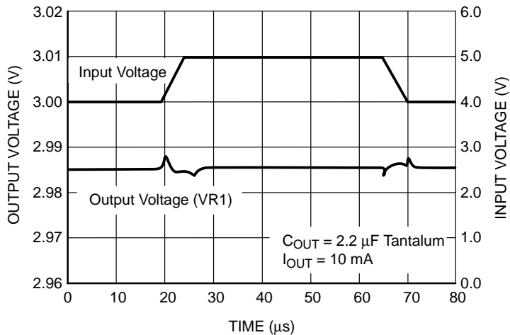
Figure 41. Line Transient Response
