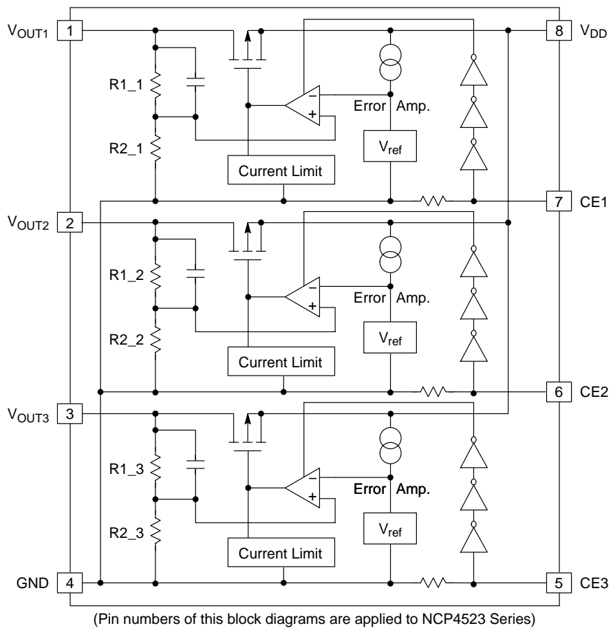
Figure 1. Block Diagram
