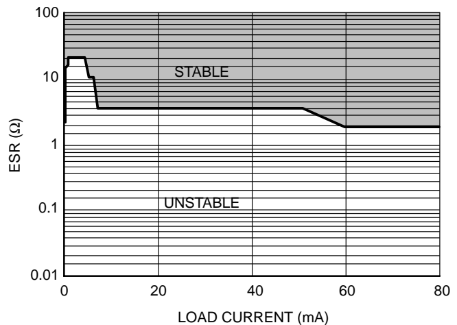
Figure 57. Ceramic Capacitor 2.2 \mu\text{F}
