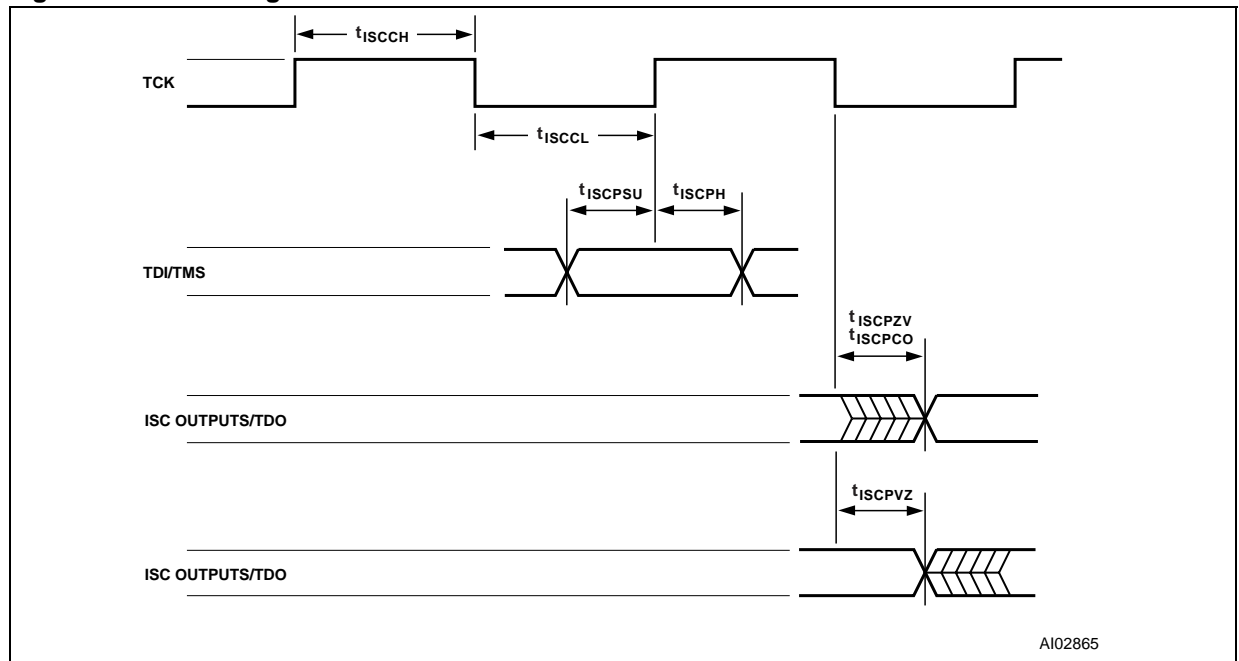
Figure 49. ISC Timing
