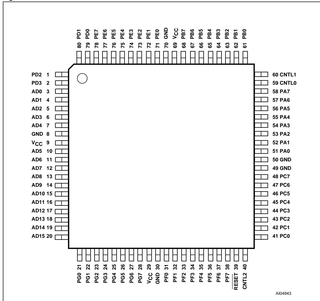
Figure 3. TQFP Connections
