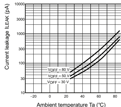
Current leakage vs. Ambient temperature I_{LEAK} - T_a
