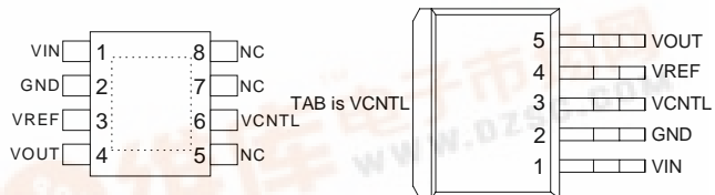
SOP-8-P (Top View)
