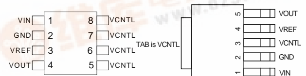
SOP-8 (Top View)
