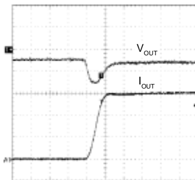
I_{OUT} = +10mA \rightarrow +3A
