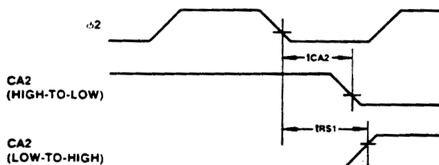
Figure 4. CA2 Timing
