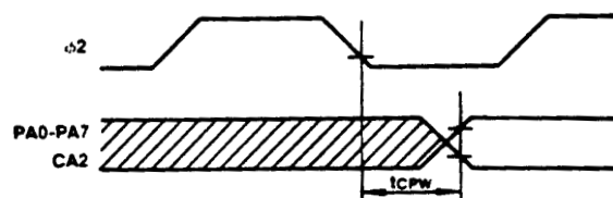
Figure 8. PA Port Delay Time
