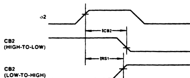
Figure 6. CB2 Timing
