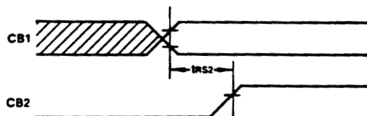
Figure 7. CB1/CB2 Handshake Timing
