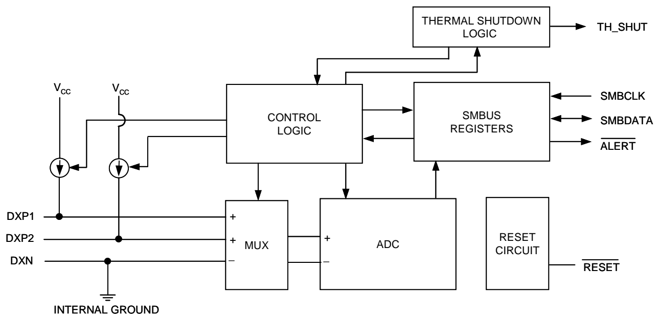
Fig 1. Functional Diagram
