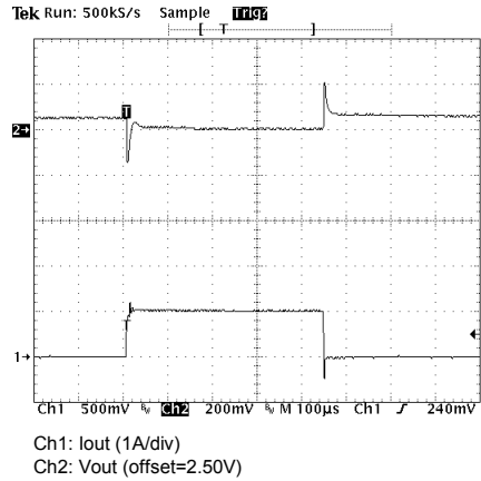
Load Transient
