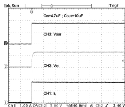
Start-UP
