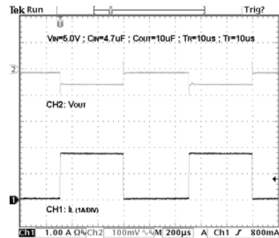
Load Transient
