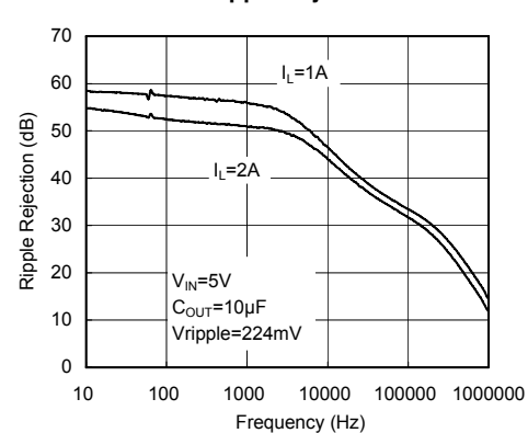
Ripple Rejection
