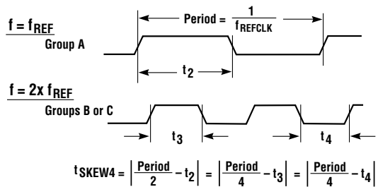
Figure 8. t_{SKEW4}
