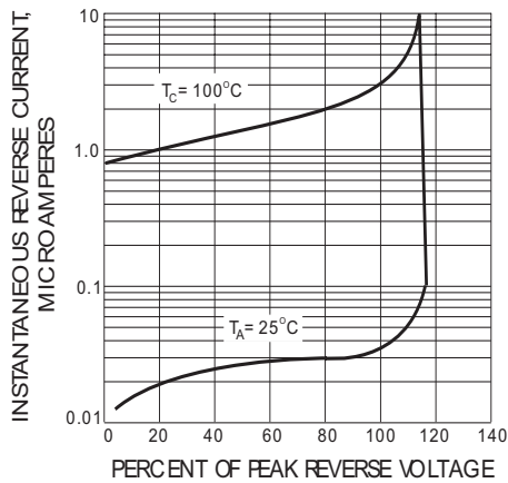
Fig. 3- TYPICAL REAK REVERSE CHARACTERISTICS
