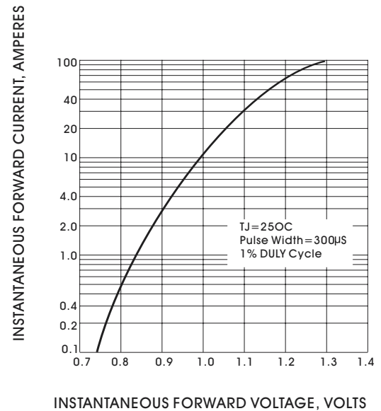
Fig. 2- TYPICAL INSTANTANEOUS FORWARD CHARACTERISTICS PER ELEMENT
