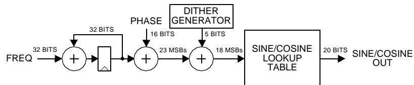
Figure 6. NCO Circuit
