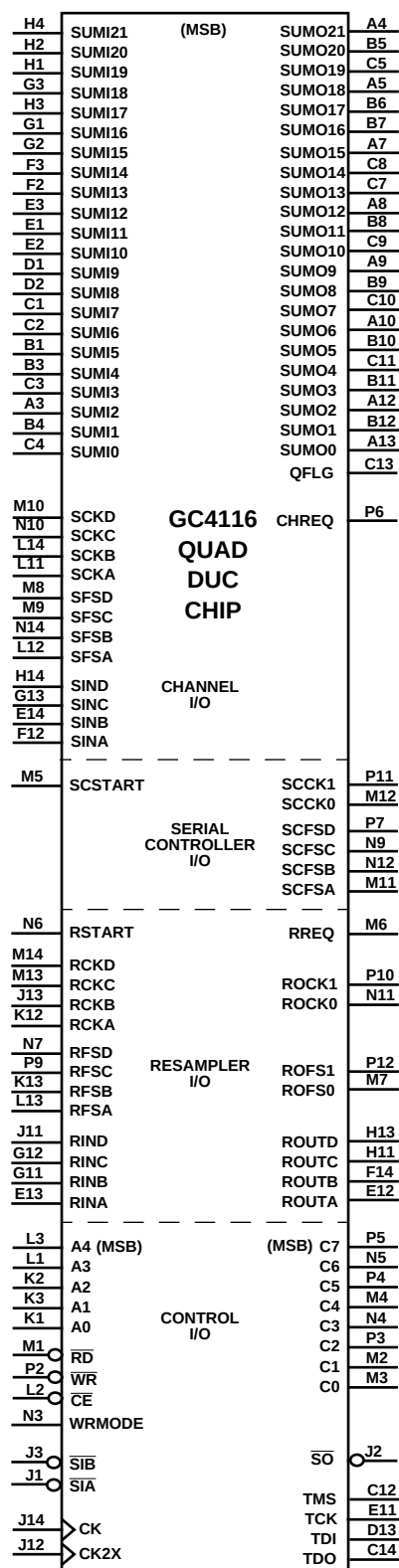
Figure 15. 160 Pin Plastic Ball Grid Array (PBGA) Package
