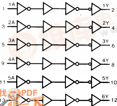
Fig. 1 Logic Diagram
