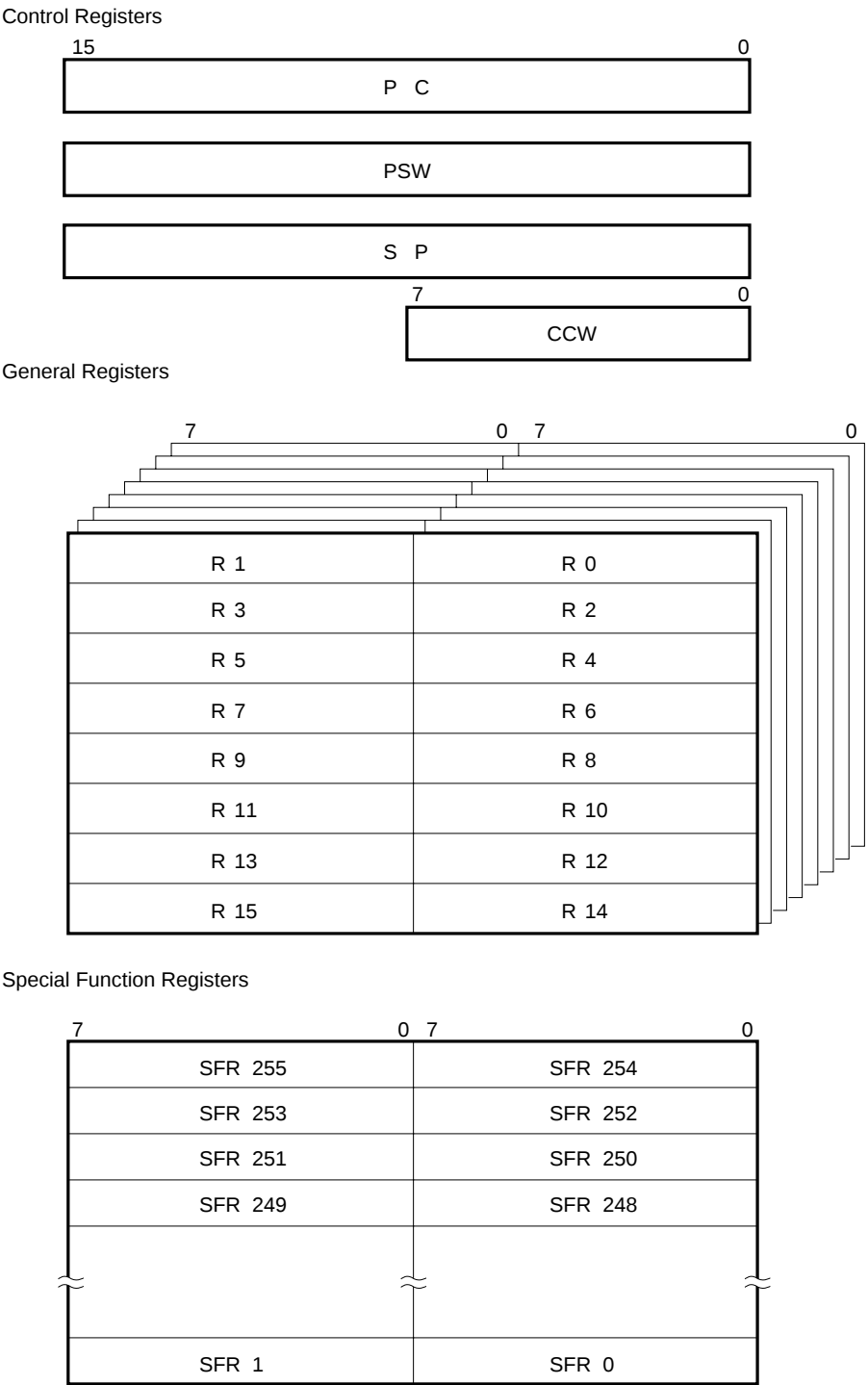
Figure 2-2. Register Configuration
