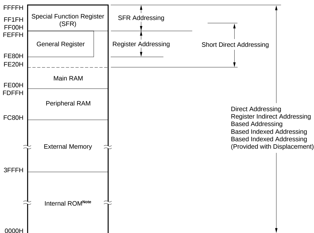
Figure 2-6. Data Memory Addressing
