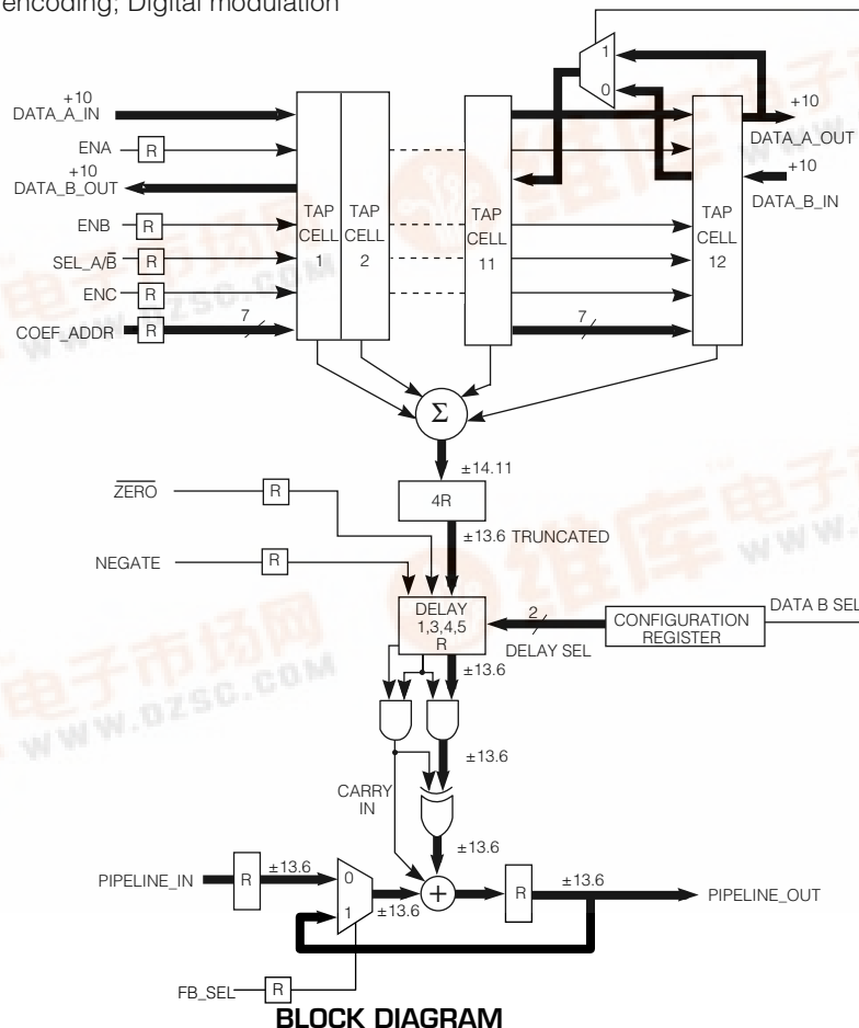
BLOCK DIAGRAM
