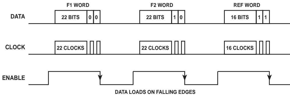
Fig. 6d Data load sequence
