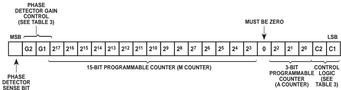
Fig. 6b F1 or F2 word, bit allocation with ÷8/9 selected
