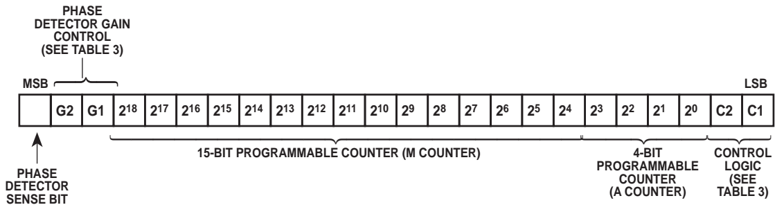
Fig. 6a F1 or F2 word, bit allocation with ÷16/17 selected
