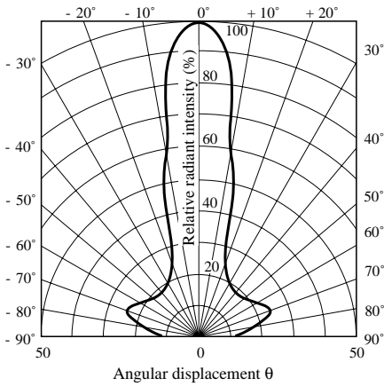
Fig. 10 Radiation Diagram
