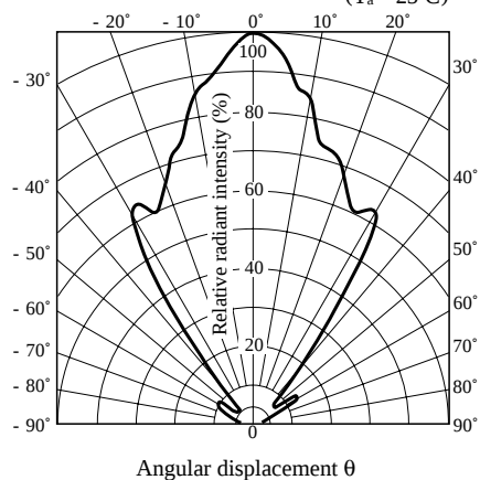
Fig. 9 Radiation Diagram
