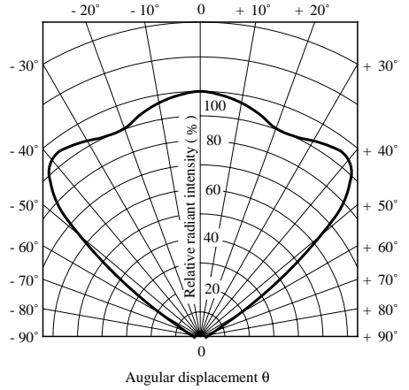
Fig.12 Radiation Diagram (GL513F) ( T_a = 25^\circ\text{C} )
