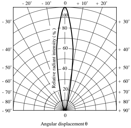
Fig.11 Radiation Diagram (GL514) ( T_a = 25^\circ\text{C} )
