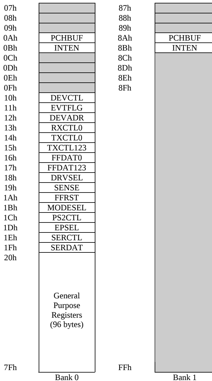
Figure 4-2 Data Memory Space
