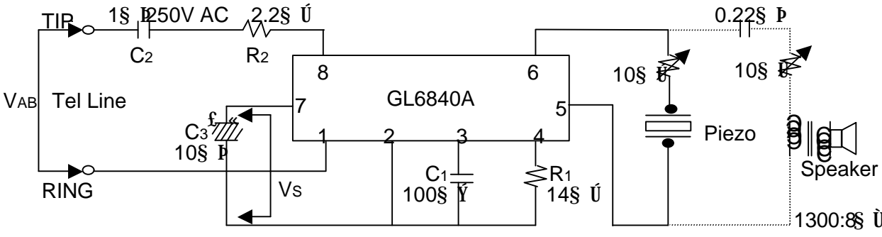
Figure3 : Differential output
