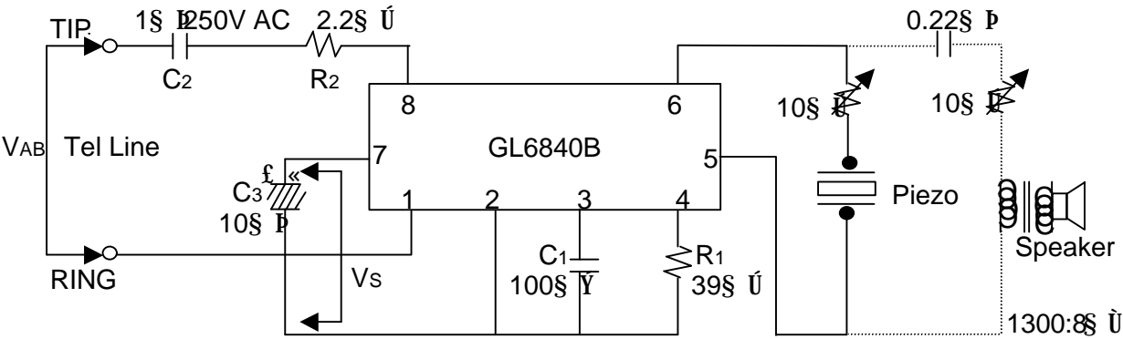
Figure3 : Differential output
