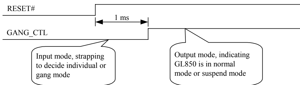
Figure 5.5 - Timing of PGANG/SUSPND strapping
