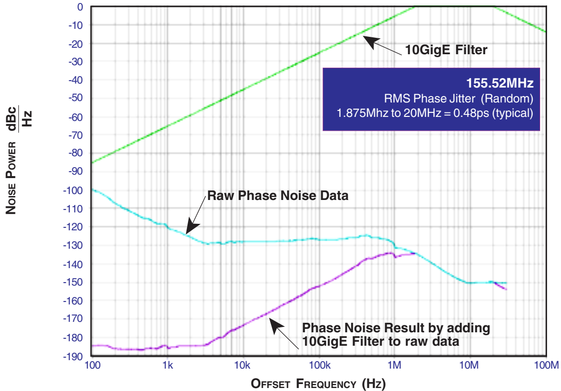
TYPICAL PHASE NOISE AT 155.52MHz
