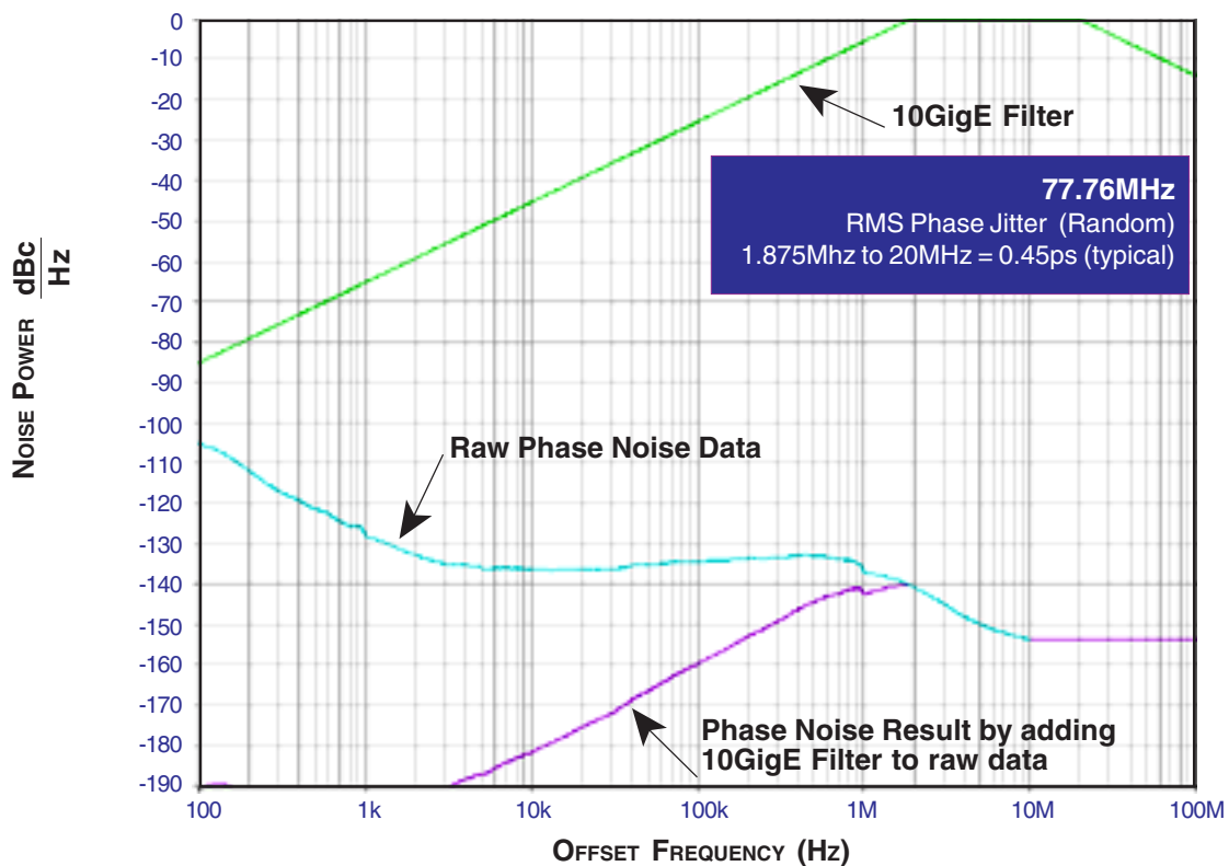
TYPICAL PHASE NOISE AT 77.76MHz
