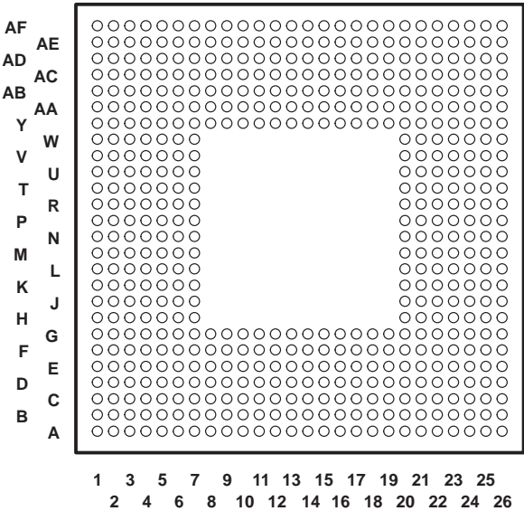
GLZ and ZLZ 532-PIN BALL GRID ARRAY (BGA) PACKAGES (BOTTOM VIEW)
