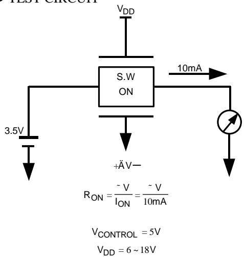
Fig.3-Ron measurement
