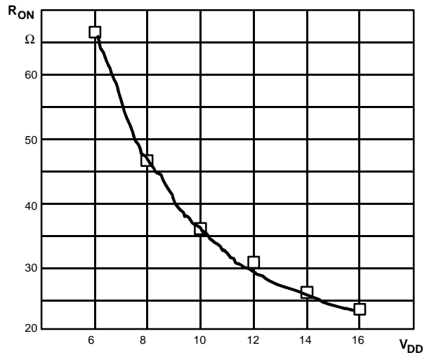
Fig.3-Ron measurement
