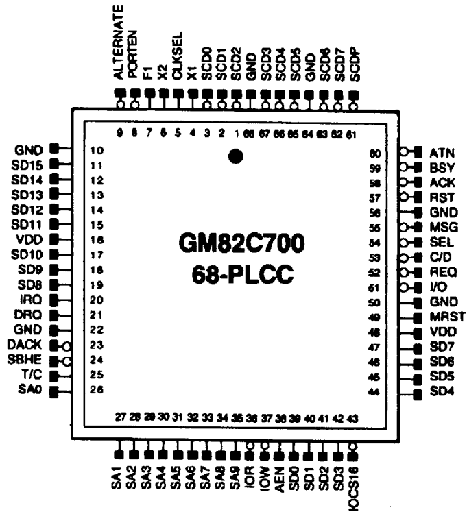
Figure 2.2 Pinout for 68-pin PLCC
