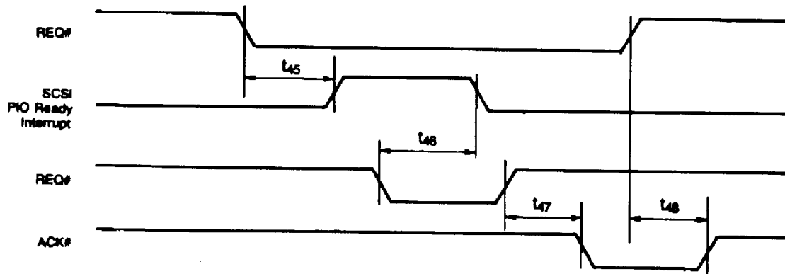
Fig 10. SCSI PIO Timing
