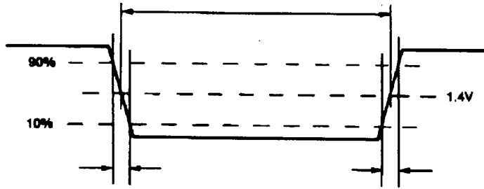
Fig 1. AC Input Conditions
