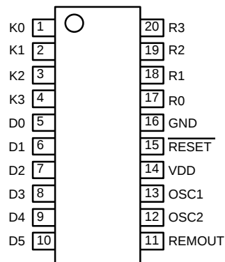
Fig 1-3 GMS34012/112 Pin Assignment
