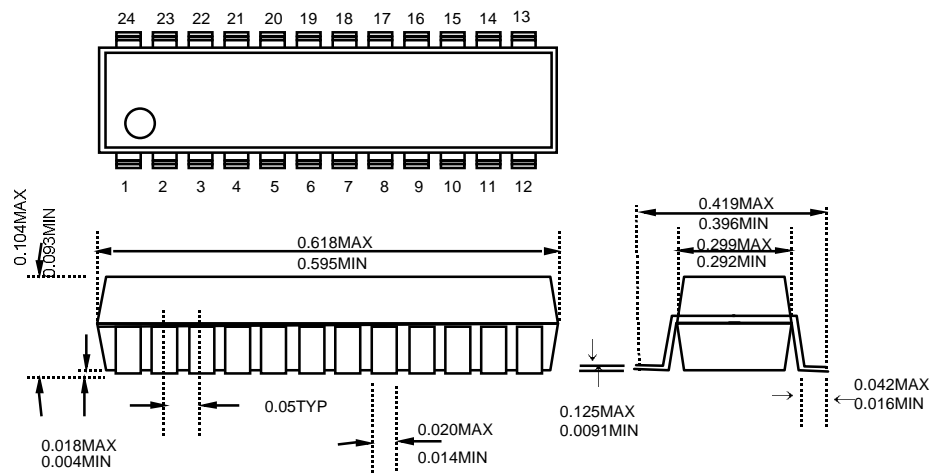
Outline (Unit : Inch)
