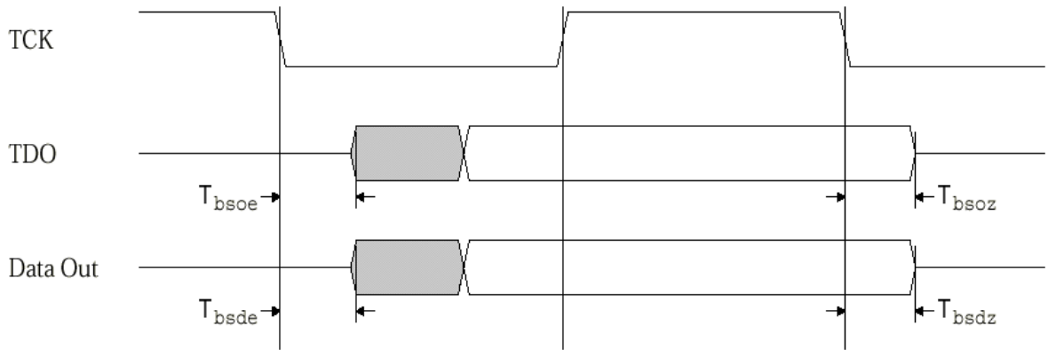
Figure 14-4: Boundary Scan Tristate Timing
