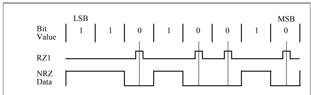
Figure 12-7: RZI/NRZ bit encoding example
