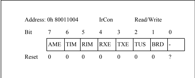
Figure 12-3: Location of bits within Ir Control Register
