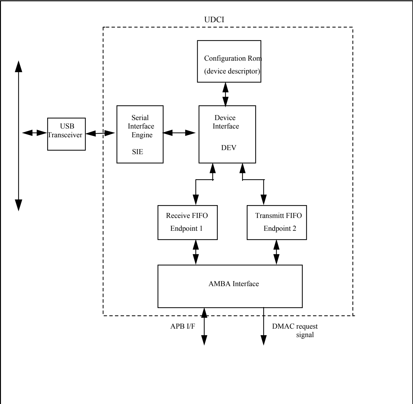
Figure 12-16: USBBD Block Diagram
