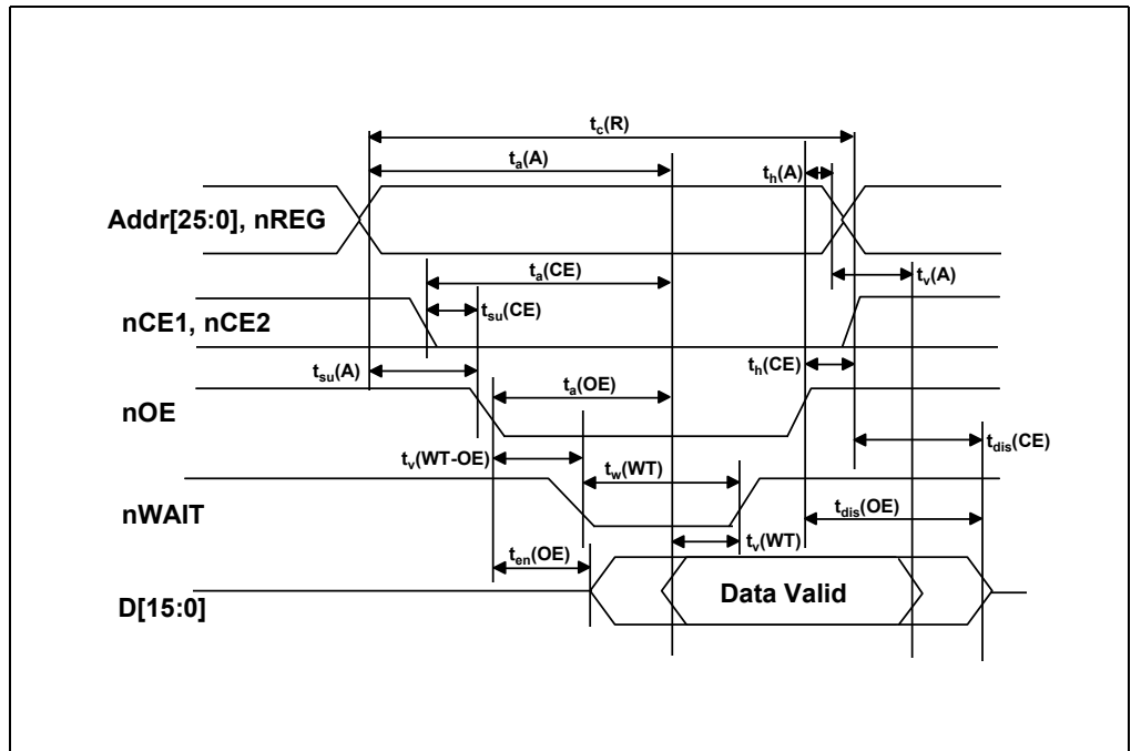
Figure 10-5: Read timing diagram
