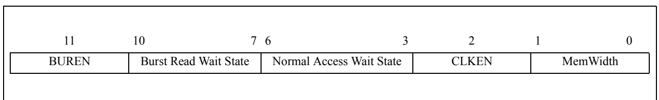
Figure 9-2: Byte fields in the memory configuration register
