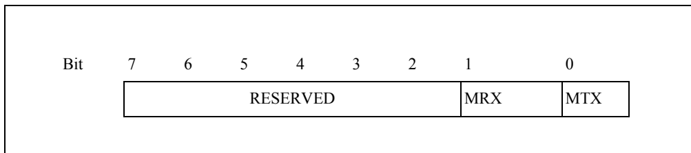
Figure 12-31: DMAC request masking register
