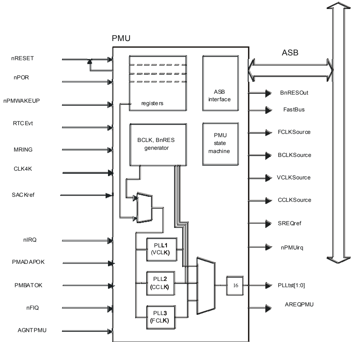
Figure 7-1: Block Diagram
