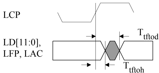
Figure 15-7: TFT mode Signal delay
