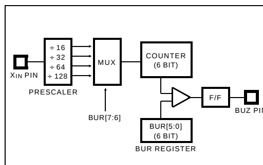
Figure 25. Buzzer Driver
