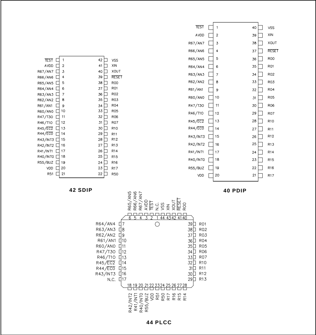
Figure 2. Pin Connections
