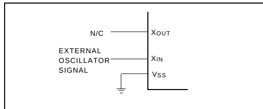
Figure 45. External Clock Drive Configuration
