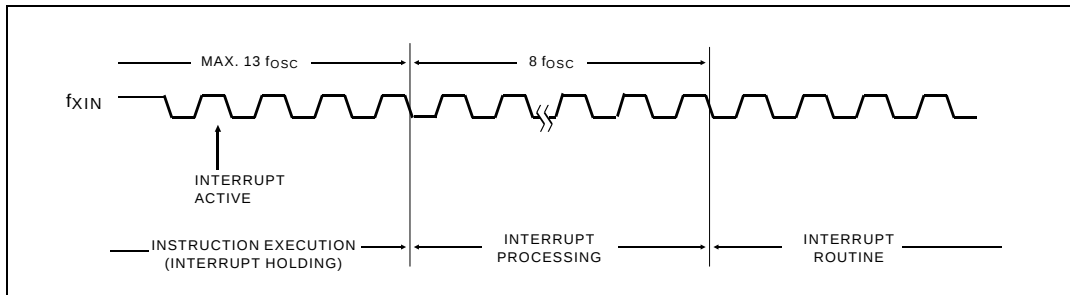
Figure 31. INT Pin Interrupt Timing
