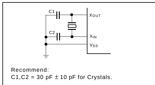
Figure 44. Oscillator Connections
