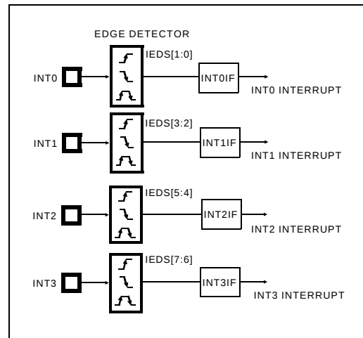
Figure 30. External Interrupt
