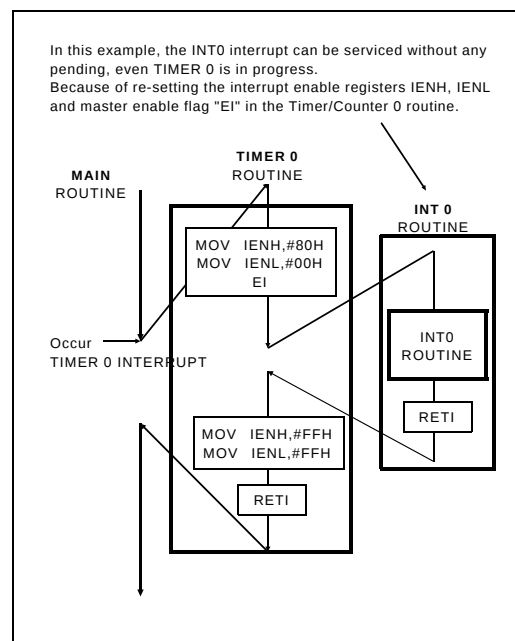
Figure 34. Execution of Multi-Interrupt
