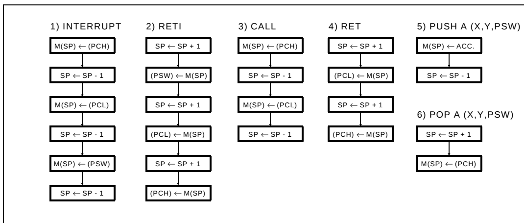
Figure 7. Stack Operation
