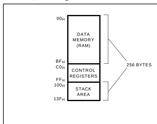
Figure 9. Data Memory
