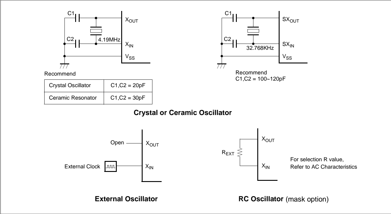
Figure 18-1 Oscillation Circuit
