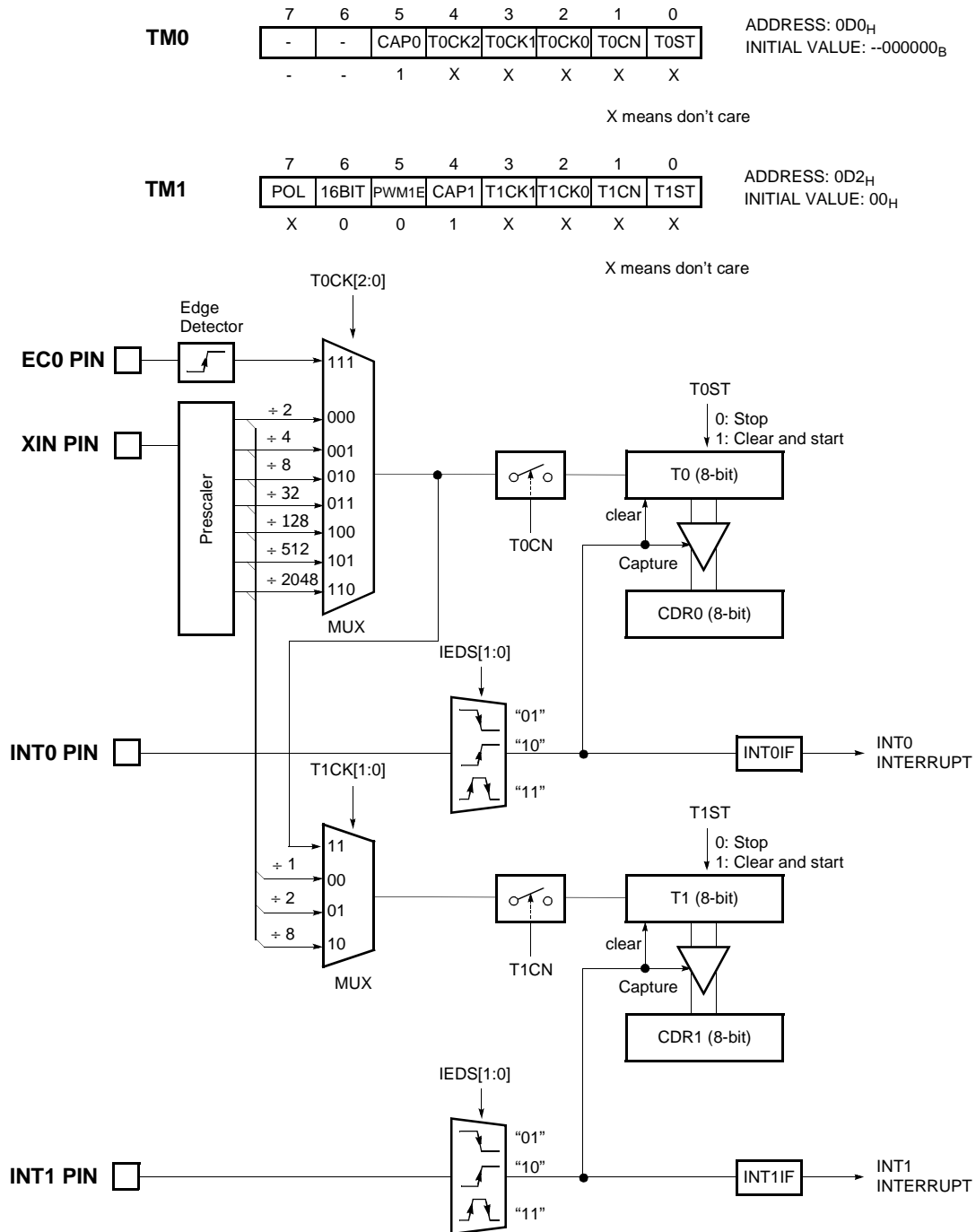
Figure 12-8 8-bit Capture Mode
