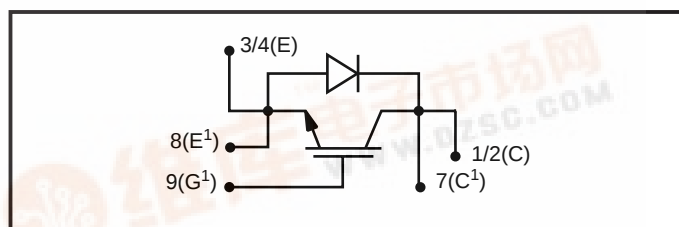
Fig.2 Single switch circuit diagram
