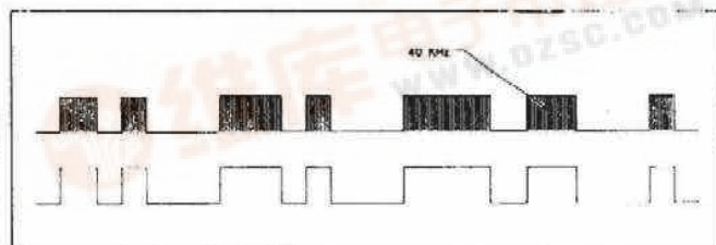
Timing Diagram
