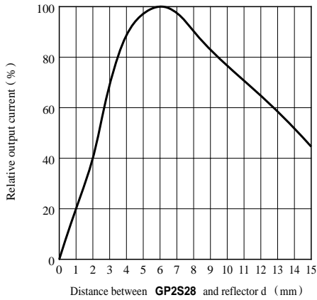
Fig. 9 Relative Output Current vs. Detecting Distance
