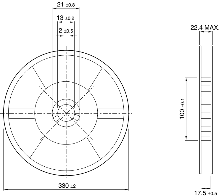
Figure 15. Reel Structure and Dimensions
