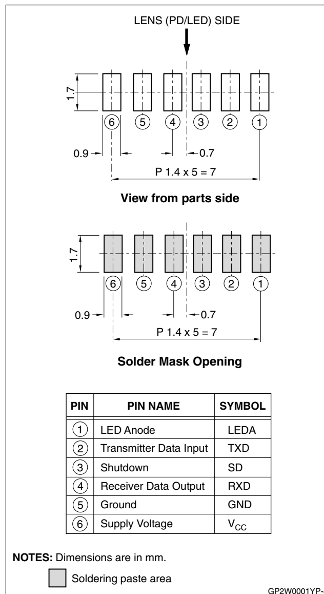
Figure 4. Foot Pattern and Solder Cream Paste Size
