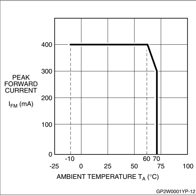
Figure 12. Peak Forward Current Versus Ambient Temperature
