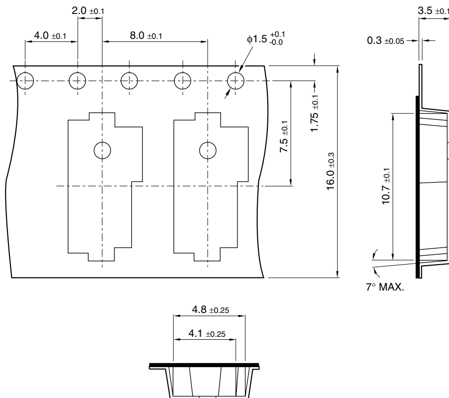
Figure 14. Tape Structure and Dimensions
