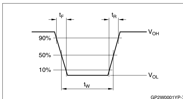
Figure 7. Output Waveform (Detector Side)
