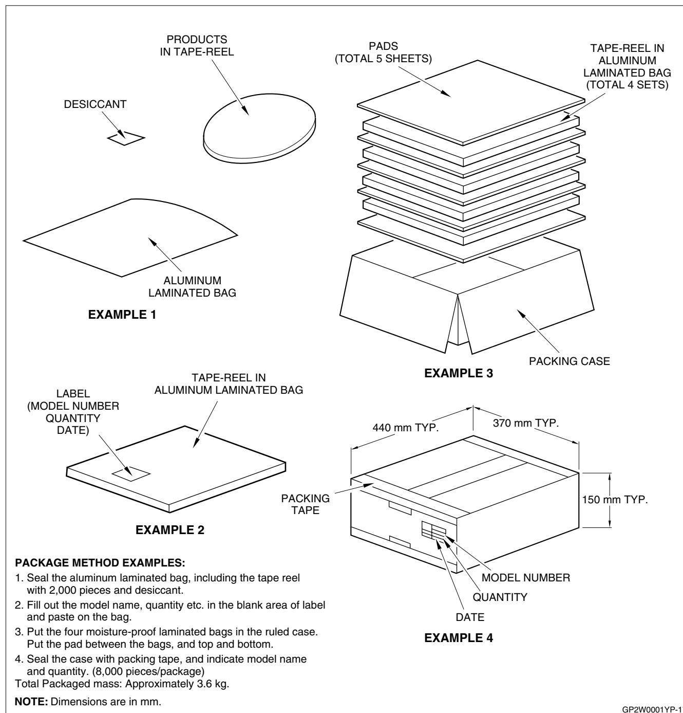
Figure 17. Packing Specification
