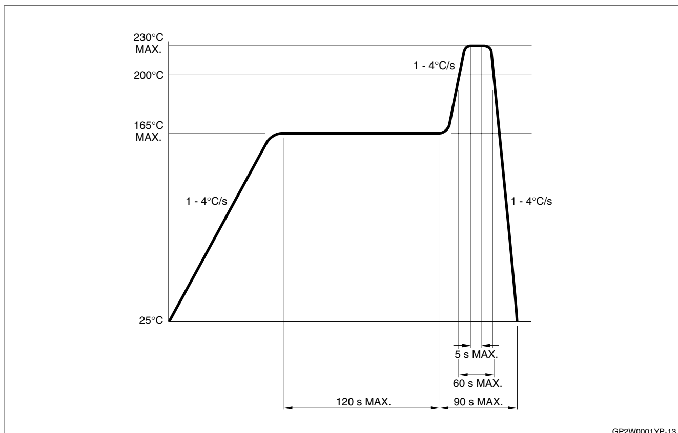
Figure 13. Temperature Profile
