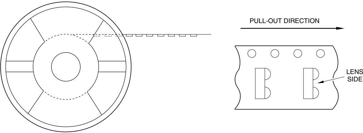
Figure 16. Direction of Product Insertion
