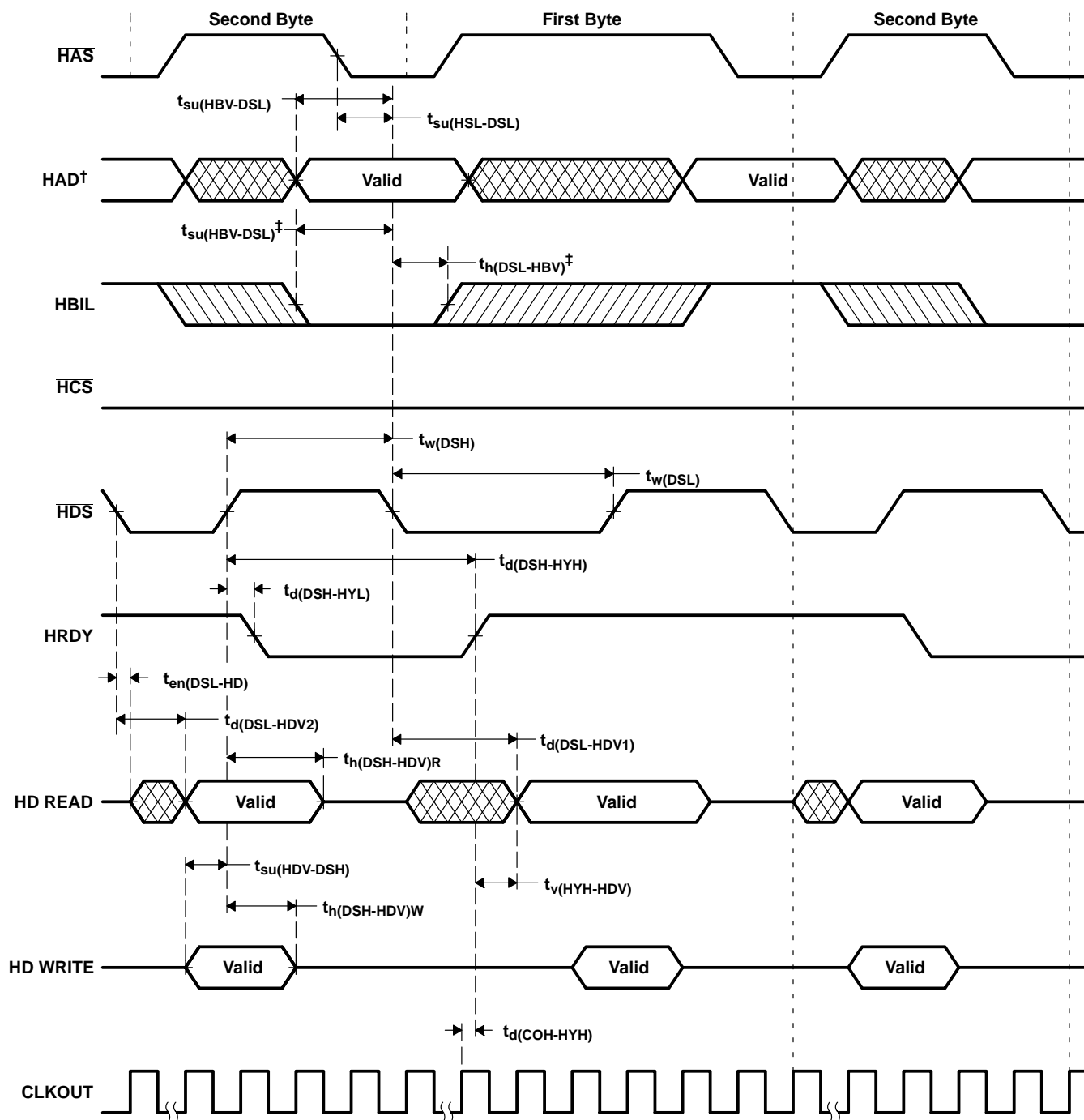
Figure 6-27. Using HDS to Control Accesses (HCS Always Low)
