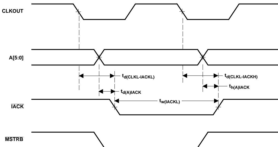
Figure 6–17. \overline{\text{IACK}} Timings
