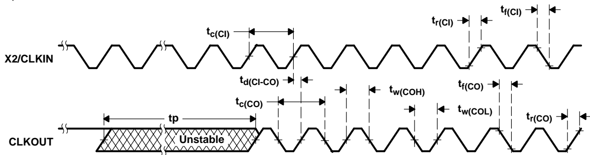
Figure 6–4. External Multiply-by-One Clock Timing
