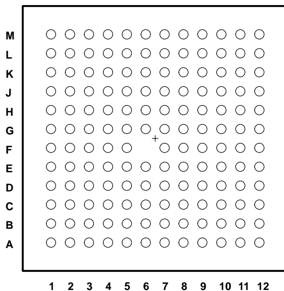
Figure 2-1. 143-Terminal GQW and ZQW Ball Grid Array (Bottom View)
