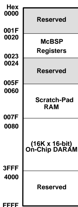
Figure 3–8. HPI8 Memory Map
