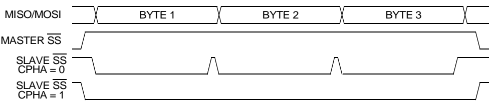
Figure 20-12CPHA/SS Timing
