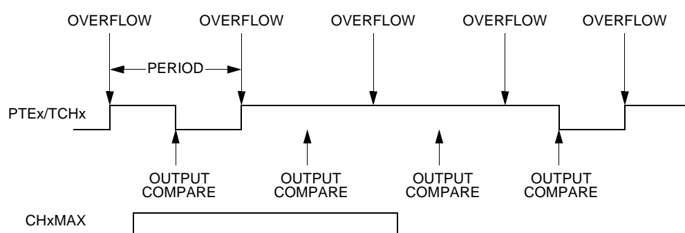
Figure 22-13. CHxMAX Latency
